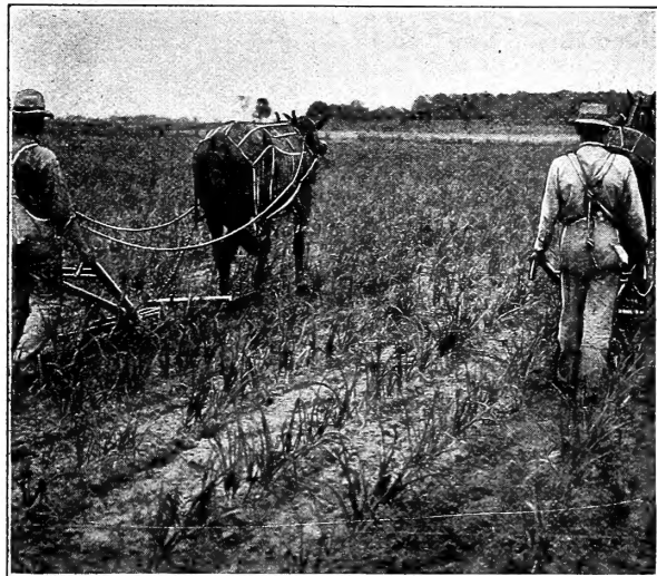
The Planet Jr. Horse Hoe Cultivating in the Field
